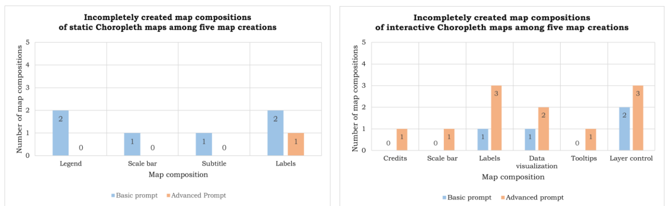
Figure 48 The number of map compositions of static (left) and interactive (right) choropleth maps that were unsuccessfully created among five iterations.
