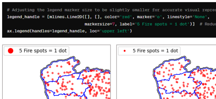
Figure 20 refined code and adjusted legend dot sizes
